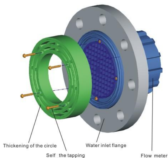
Figure 21: GL40\GL50 Thickening of the inlet butterfly valve
