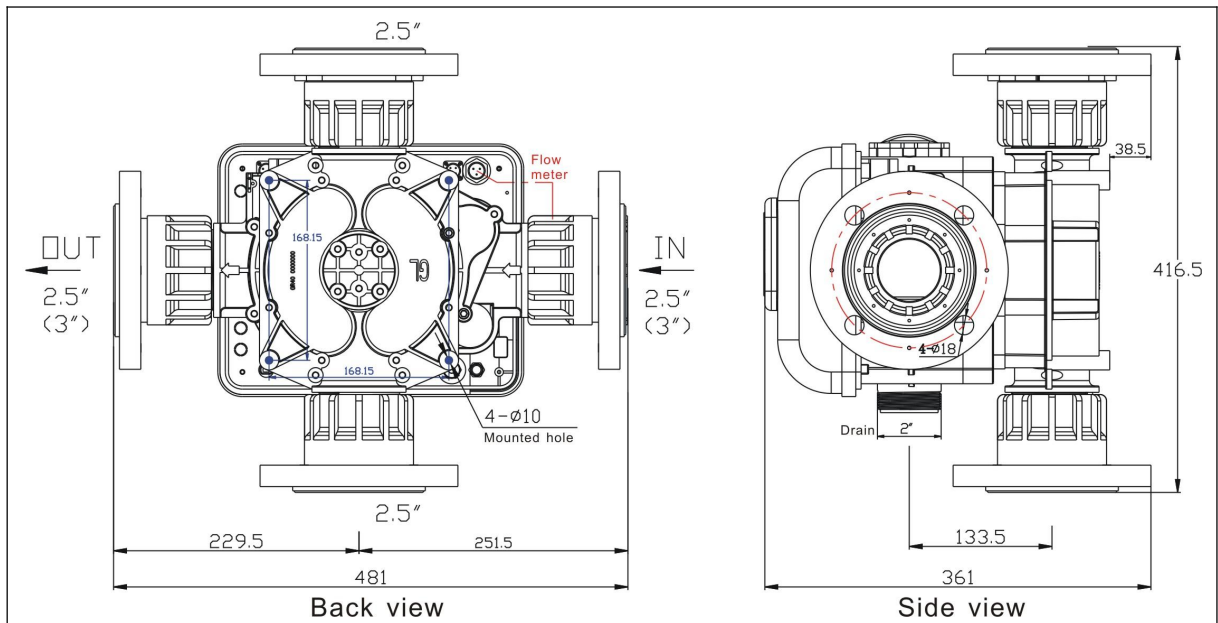
Figure 12: GL40 valve body geometry size
